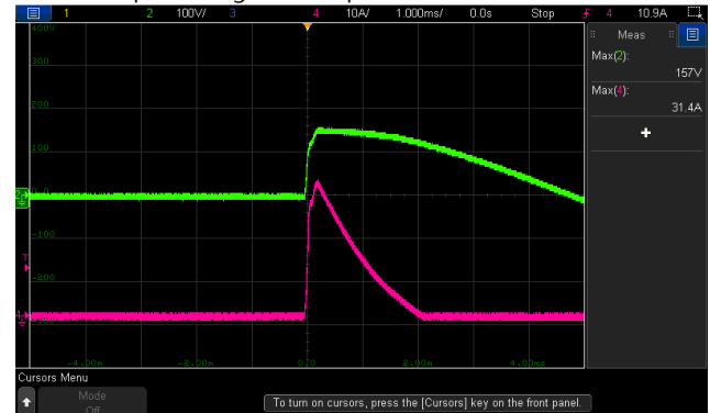
INPUT=115VAC/ 60HZ @ FULL LOAD CH1: AC Input Voltage CH2: Input current
