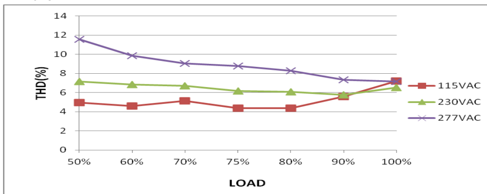
THD vs LOAD
